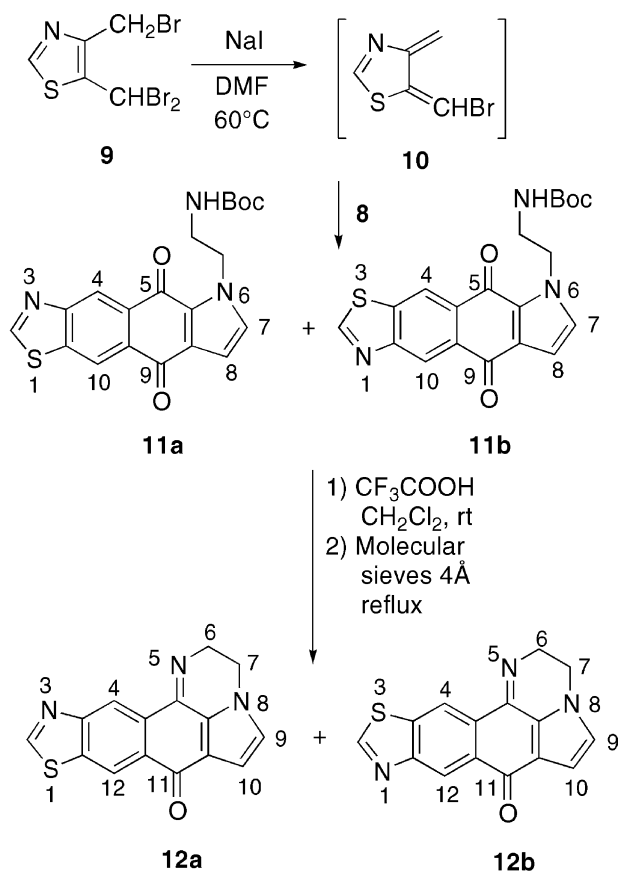
Scheme 3. Regioisomers ratio: 11a/11b = 52/48; 12a/12b = 52/48.
