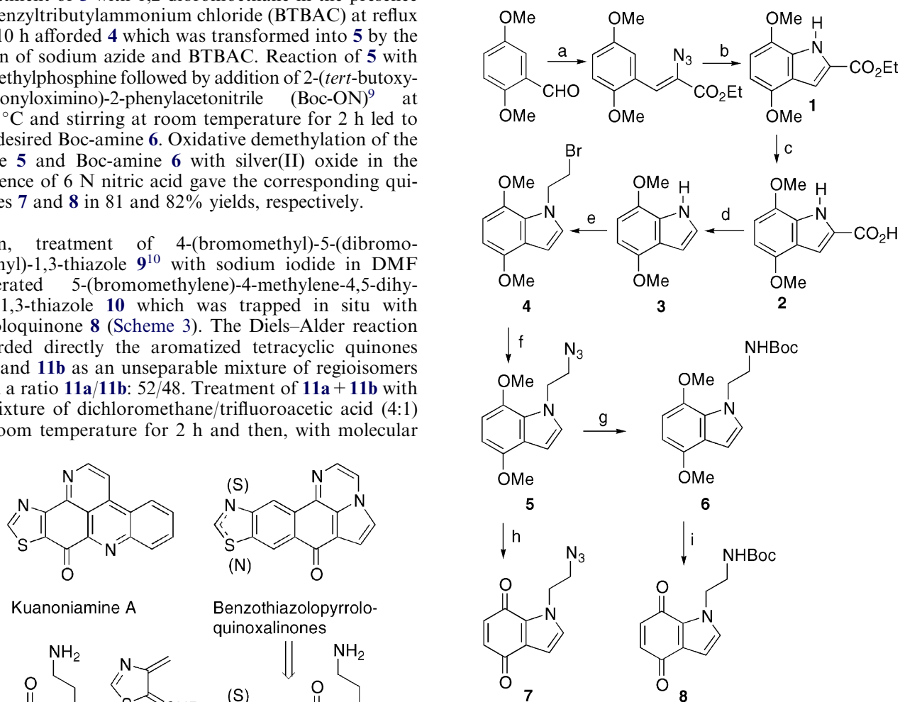
Scheme 2. Reagents and conditions: (a) Na, EtOH, N 3 CH 2 CO 2 Et, –10 °C, rt, 2 h, 75%; (b) toluene, reflux, 5 h, 99%; (c) 10% NaOH, reflux, 1 h, 6 M HCl, 0 °C, 90%; (d) Cu, quinoline, N 2 , 150–160 °C, 3 h, 95%; (e) Br–CH 2 –CH 2 –Br, NaOH, BTBAC, reflux, 10 h, 74%; (f) NaN 3 , BTBAC, reflux, 20 h, 93%; (g) Me 3 P, Boc-ON, –10 to 0 °C, 1 h, rt, 2 h, 76%; (h) AgO, HNO 3 , rt, 15 min, 81%; (i) AgO, HNO 3 , –10 °C, 1 min, 82%.
